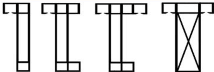
Single Track Single Gate 3' to 22' Single Track Single Gate Strengthened 23' to 30' Dual Track Single Gate 23' to 30' Box Frame
